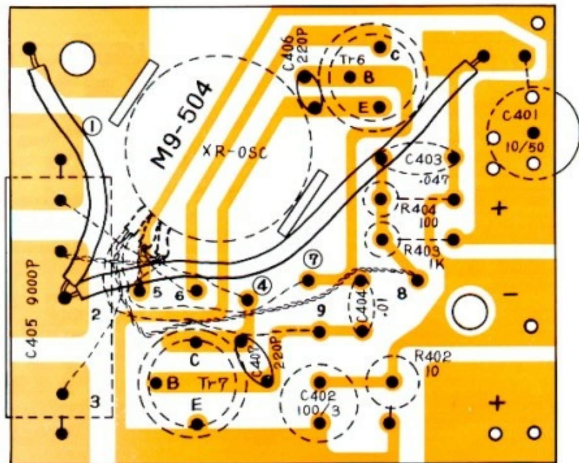
Tr 6, 7. 2SC696(J)(IXF)
