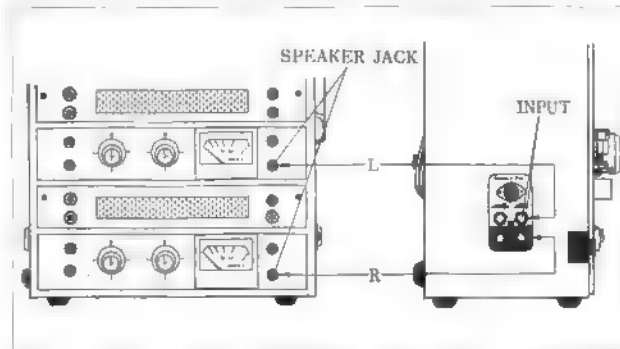
Connecting AKAI M-Series Tape Recorder with X-150D.
